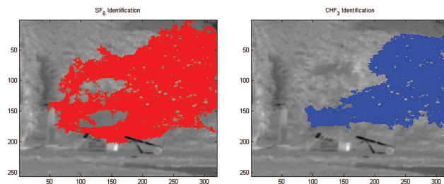
Fig. 10. (Color online) Result of the identification stage of the detection algorithm for \text{CHF}_3 and \text{SF}_6 plumes, released simultaneously.
